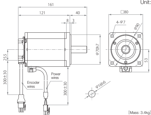
GYS motor (without brake)
