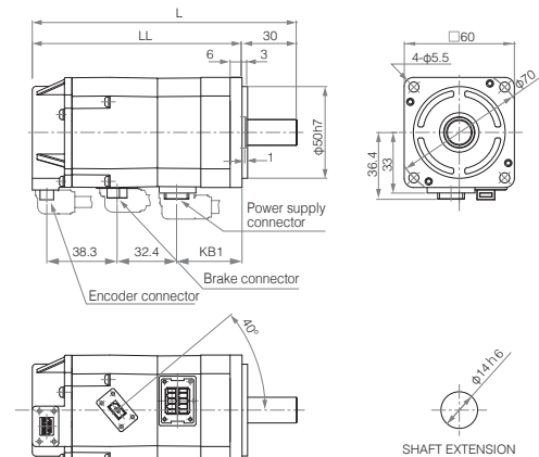
GYB motor (with brake)
