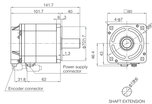
GYB motor (without brake)
