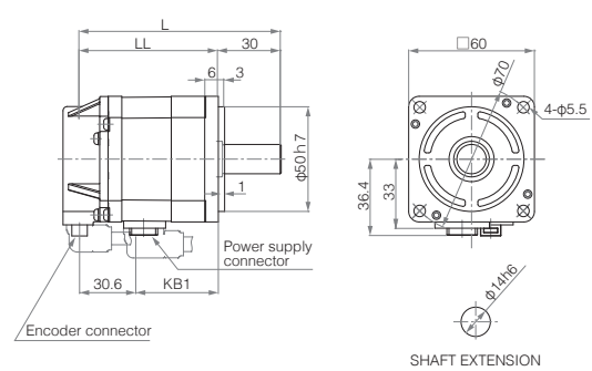
GYB motor (without brake)
